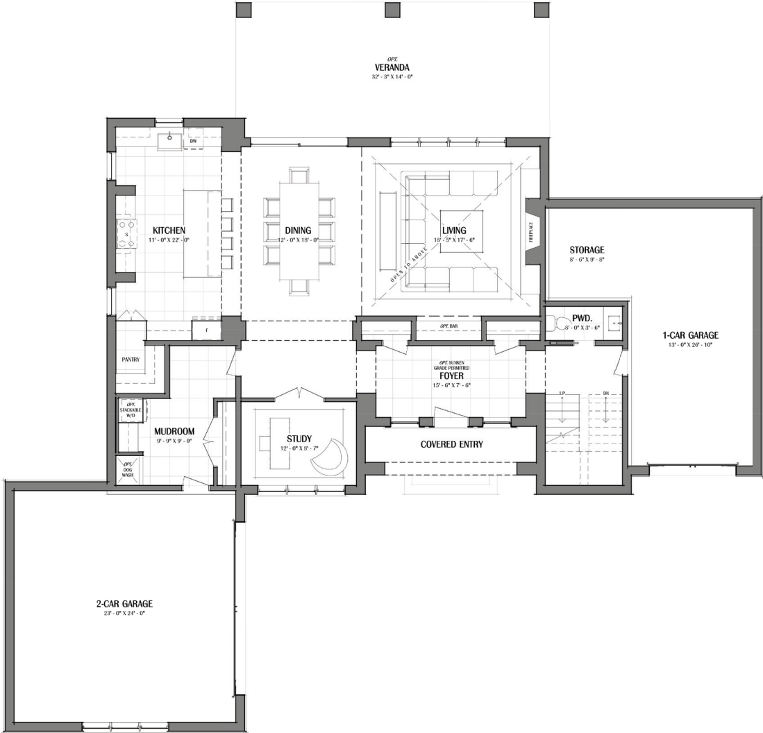
FIRST FLOOR
