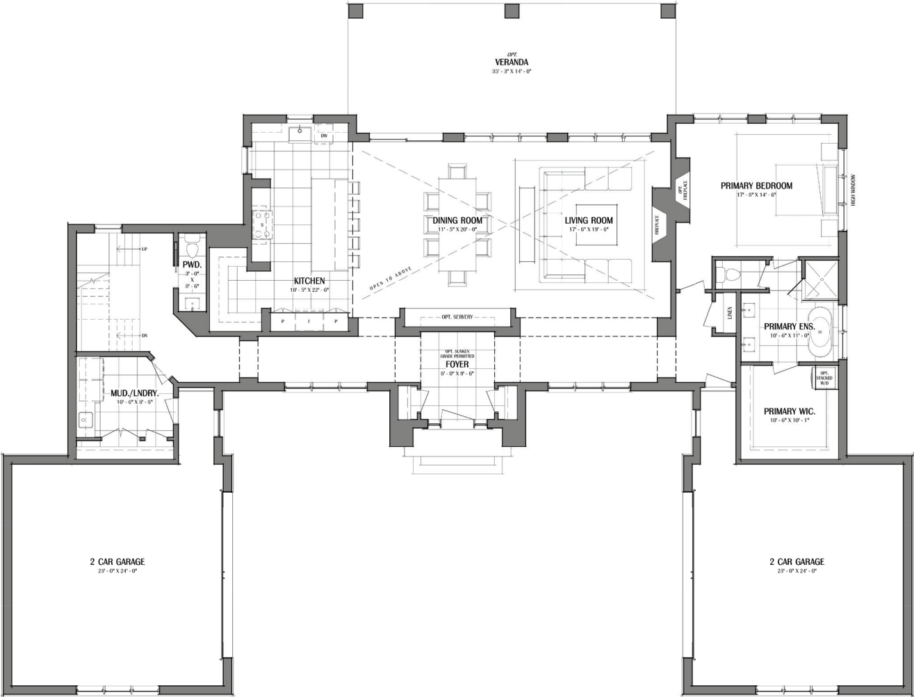
FIRST FLOOR
