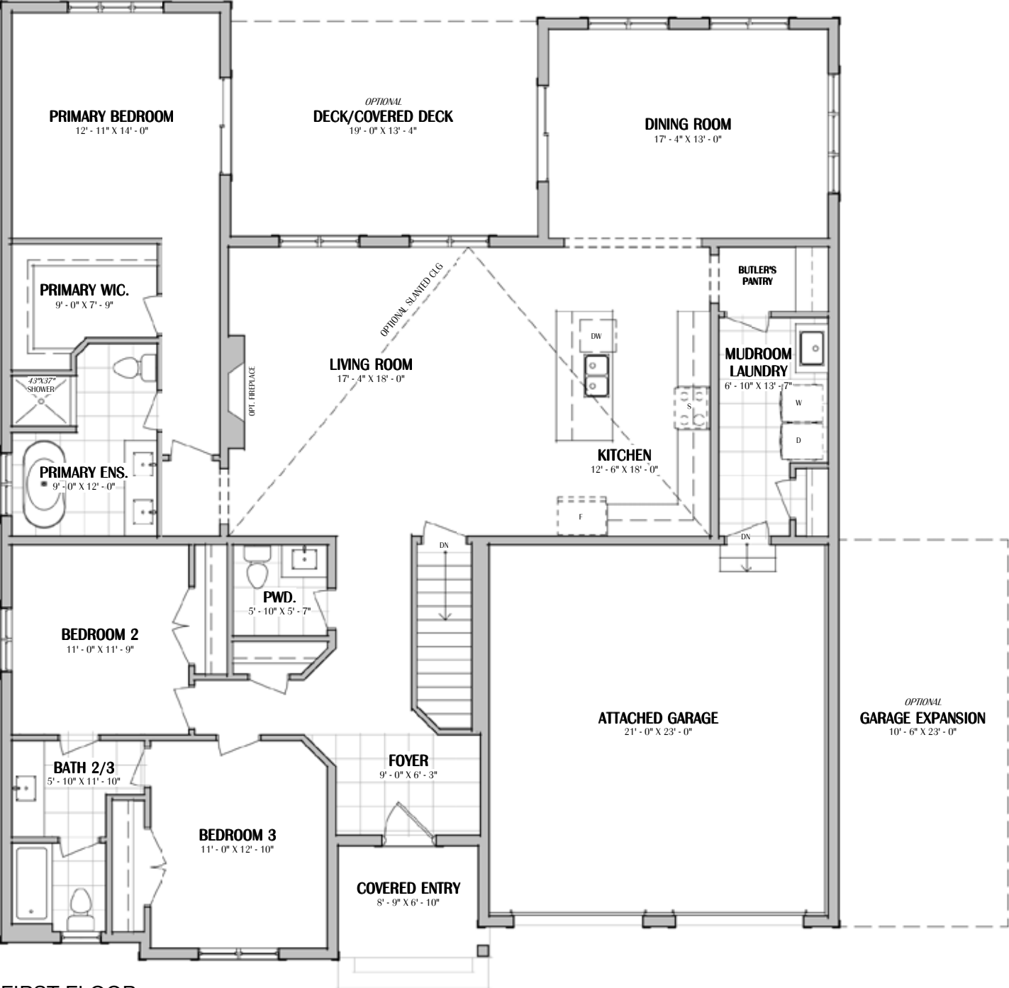
FIRST FLOOR
